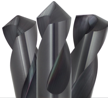
SD SERIES 2 Flute 30° Helix 90°, 120° & 150° point angle P M K S H N Varianta Supral Coating
