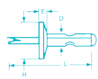
Countersunk
