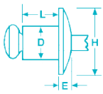
Buttonhead
